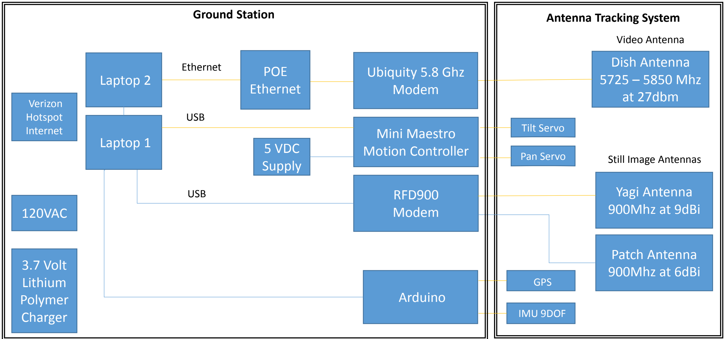
Basic Primary Payload Ground Station Block Diagram Rev 2 (11/19/15)
